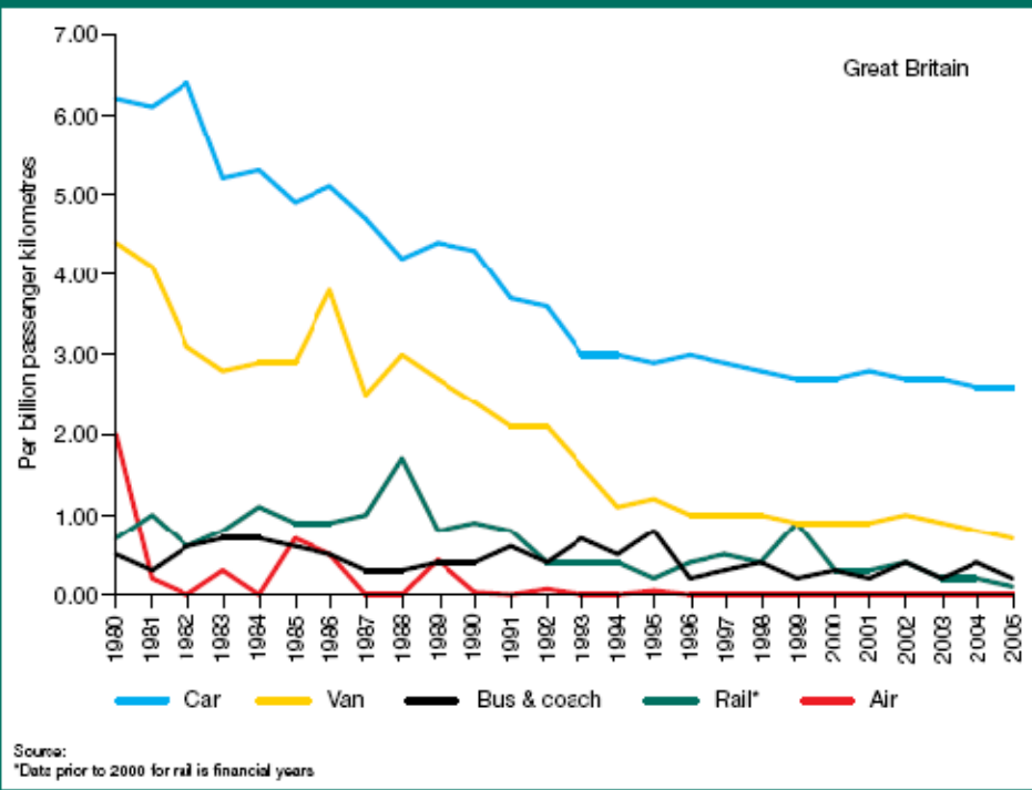
Figure 2.4: Passenger fatality rates in air, rail, motor vehicles: 1980 to 2005
